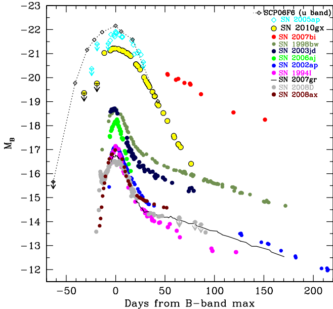
Figure 2. B -band absolute light curves of SN 2010gx (Vega system) and a number of ultra-bright events and canonical stripped-envelope SNe, including the type Ic SNe 1994I (Richmond et al. 1996, and references therein), 2002ap (Pandey et al. 2002; Foley et al. 2003; Yoshii et al. 2003; Tomita et al. 2006), 2006aj (Campana et al. 2006; Cobb et al. 2006; Mirabal et al. 2006; Pian et al. 2006; Sollerman et al. 2006), 2003jd (Valenti et al. 2008a), and 1998bw (Galama et al. 1998; McKenzie & Schaefer 1999; Sollerman et al. 2000; Patat et al. 2001); the type Ib SNe 2007gr (Valenti et al. 2008b; Hunter et al. 2009) and 2008D (Mazzali et al. 2008; Soderberg et al. 2008; Modjaz et al. 2009); the type IIb SN 2008ax (Pastorello et al. 2008). B -band light curves for the luminous SNe 2005ap, 2010gx, and 2007bi are obtained correcting the observed broadband photometry for time dilation and differences in effective rest-frame band ( K -correction). The high redshift of SCP-06F6 ( z = 1.189 ) did not allow us to compute a realistic B -band absolute light curve, so we estimated the u -band light curve (Vega system) from the i_{775} -band photometry of Barbary et al. (2009). K -corrections for the luminous objects were computed using the spectra published by Barbary et al. (2009), Quimby et al. (2007), Young et al. (2010), and this Letter.
