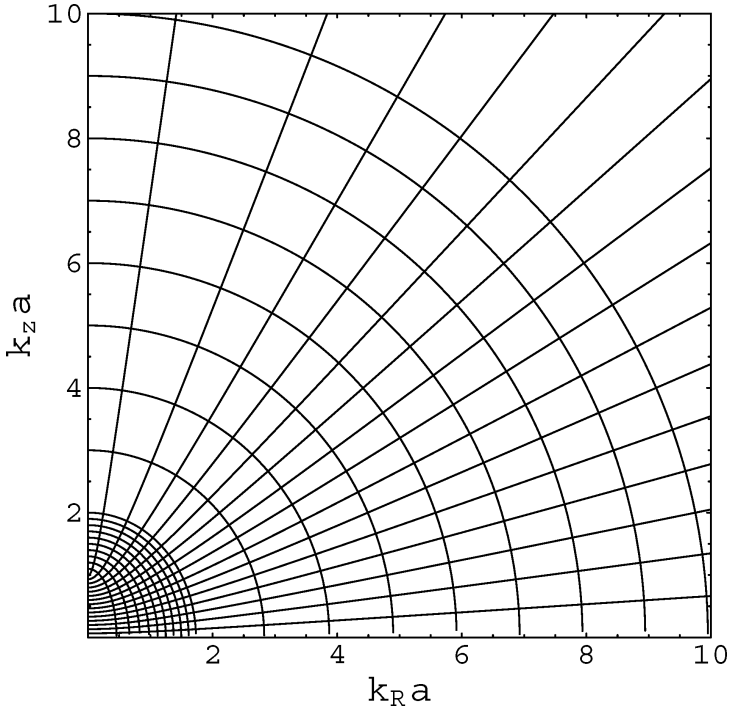
Figure 1 Contours of constant \bar{\omega} for the dispersion relation (Equation 30) of a Keplerian disk. These form a set of conformal ellipses (density waves) and hyperbolae (inertial waves). The value of \bar{\omega} along a curve is read off at the point of intersection with the k_R = 0 axis; the numerical scale is in units of \Omega = 1 . Density wave ellipses are separated by one unit for \bar{\omega} > 2 and 0.1 units for 1.1 < \bar{\omega} < 2 . Inertial wave hyperbolae are separated by .066 units.
